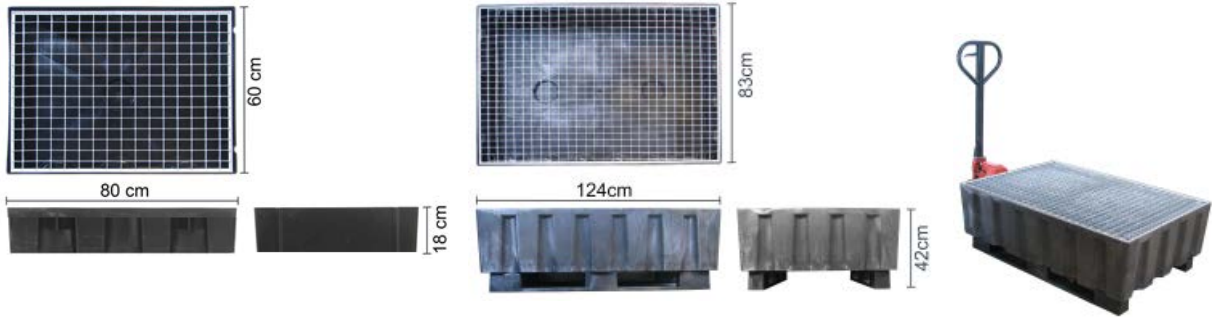
Fork lift slots
